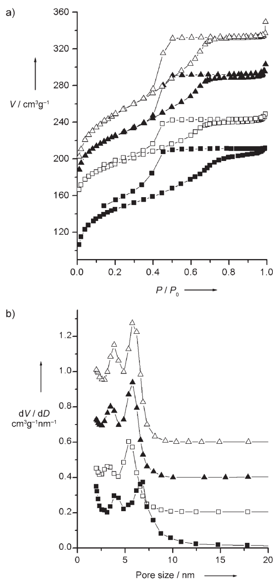
Figure 4. \text{N}_2 adsorption–desorption isotherms (a) and pore-size distribution plots (b) of FDU-17 calcined at different temperatures ( \blacksquare 450 °C; \square 600 °C; \blacktriangle 800 °C; \triangle 1000 °C). The isotherms for FDU-17-600 are offset vertically by 25 \text{ cm}^3 \text{g}^{-1} . The pore-size-distribution curves for FDU-17-600, FDU-17-800, and FDU-17-1000 are offset vertically by 0.2, 0.4, and 0.6 \text{ cm}^3 \text{g}^{-1} \text{nm}^{-1} , respectively.
